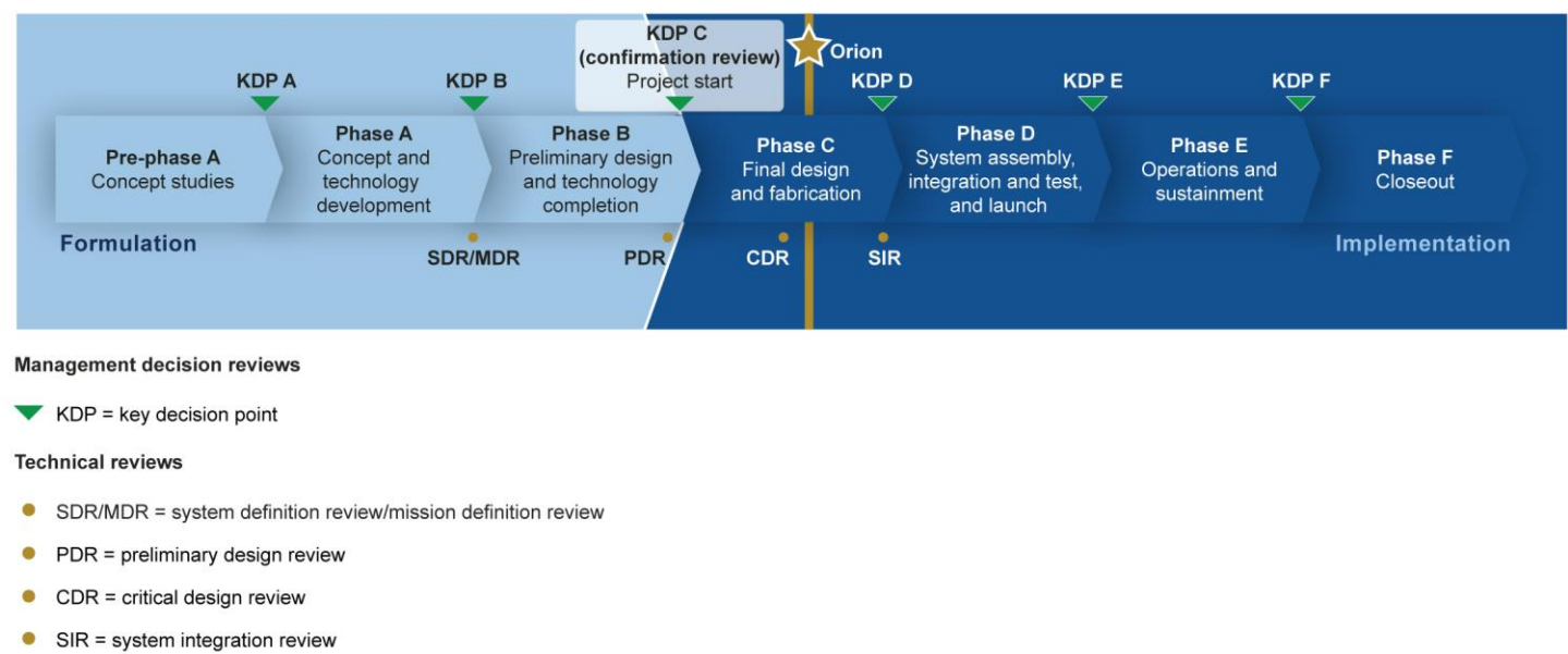
Figure 2: NASA's Life Cycle for Space Flight Projects
